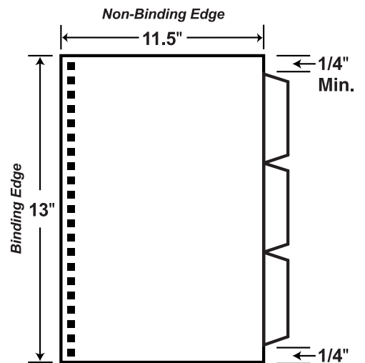
Maximum Tab Size - Automated Punch
